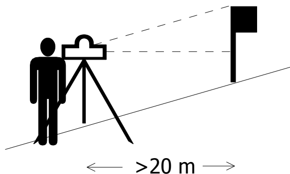
Figure A1.1 measuring the gradient of a slope with tripod-mounted sighting equipment
